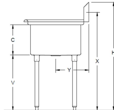
18 GAUGE 304 S/S SPACE SAVER SINK 12" DEEP - 1 COMPARTMENT
