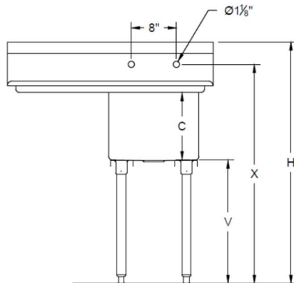
18 GAUGE 304 S/S SPACE SAVER SINK 12" DEEP - 1 COMPARTMENT
